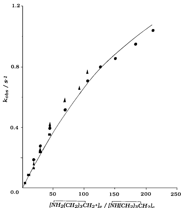
Fig. 4 Dependence of k_{\text{obs}} on [\text{NH}_2(\text{CH}_2)_3\text{CH}_2]^+ / [\text{NH}(\text{CH}_2)_3\text{CH}_2]_e for the reaction between [\text{Fe}_4\text{S}_4(\text{SEt})_4]^{2-} and \text{PhS}^- in the presence of [\text{NH}_2(\text{CH}_2)_3\text{CH}_2]^+ in \text{MeCN} at 25.0 \text{ }^\circ\text{C} {ionic strength = 0.1 \text{ mol dm}^{-3} ( [\text{NBu}^+\text{d}][\text{BF}_4]^- ); [\text{Fe}_4\text{S}_4(\text{SEt})_4]^{2-} = 0.05 \text{ mmol dm}^{-3} . Data points correspond to: [\text{NH}_2(\text{CH}_2)_3\text{CH}_2]^+ = 1.0\text{--}20.0 \text{ mmol dm}^{-3} ; [\text{PhS}^-] = 0.5 (●), 1.0 (▲) or 1.0 \text{ mmol dm}^{-3} , [\text{NH}(\text{CH}_2)_3\text{CH}_2] = 0.2 \text{ mmol dm}^{-3} (■). Curve drawn is that defined by eqn. (16) and the parameters in the text.
